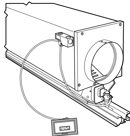
Fig. 49 — VAV Control Arrangement for Electric Warm-Up
